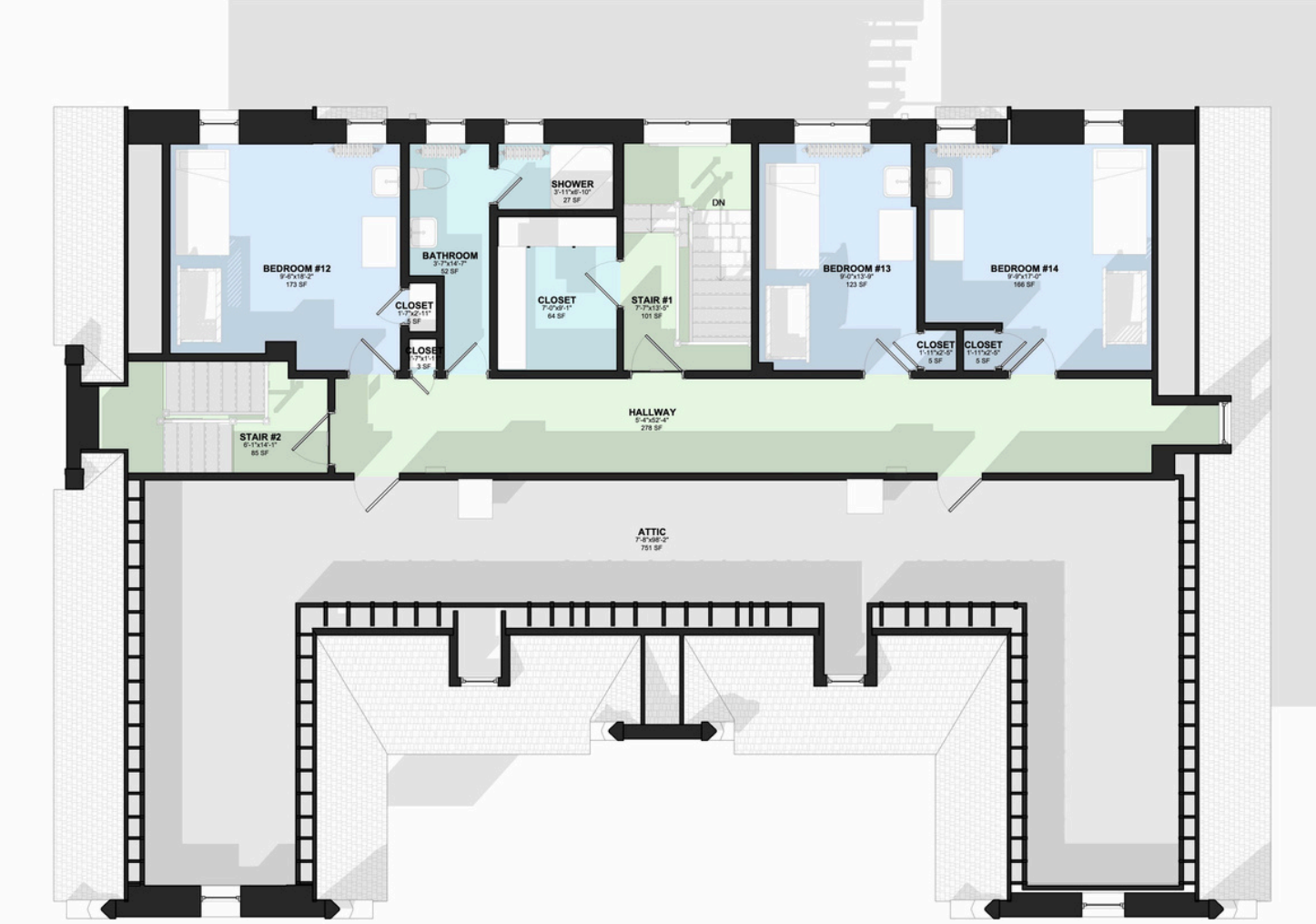
3RD FLOOR
